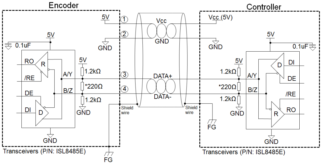
Figure 3: Circuit diagram of half-duplex transceiver
